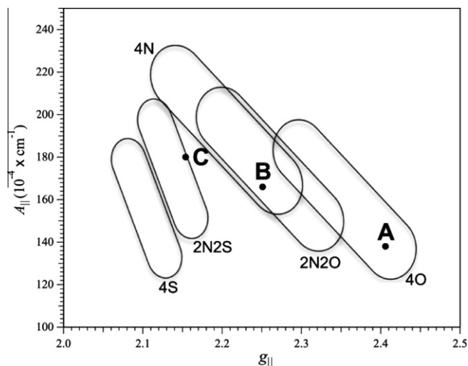
Fig. 2. Peisach and Blumberg analysis of Cu(II) EPR spectra. The regions of the plot show the likely equatorial coordination of Cu(II) for species with ranges of values of g_{\parallel} and A_{\parallel} . A corresponds to \text{CuCl}_2 , B to the intermediate species of Cu(II)–BsSCO, and C to the equilibrium species of Cu(II)–BsSCO.
