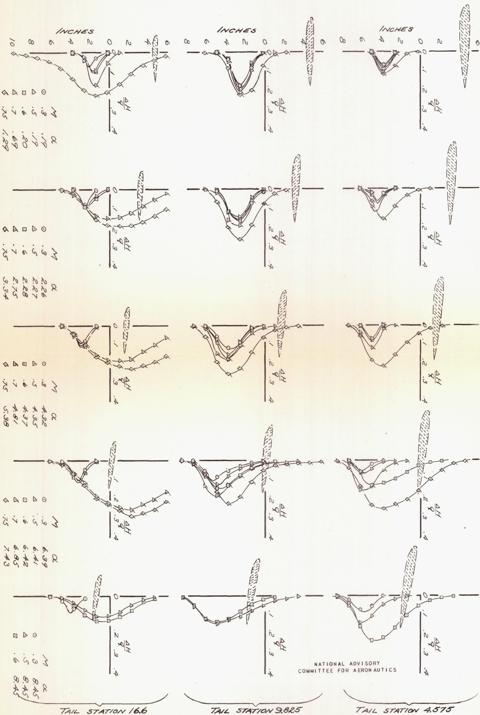
FIGURE 34. - POSITION OF WING WAKE RELATIVE TO THE TAIL AT VARIOUS MACH NUMBERS AND ANGLES OF ATTACK. WING, NACELLES, FUSELAGE, AND TURRETS AND SIGHTING DOMES.
