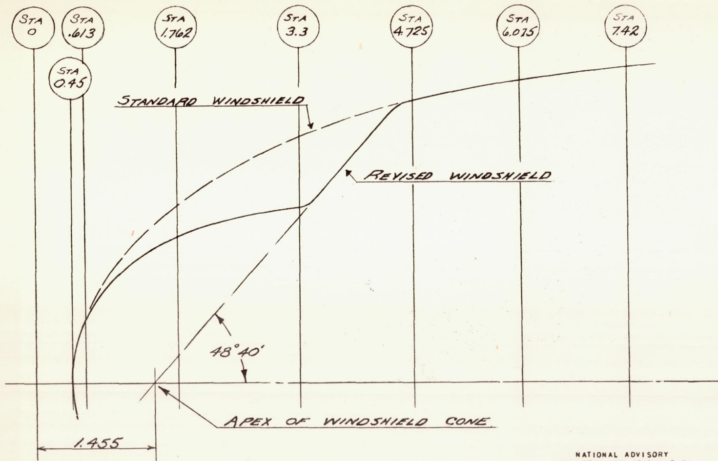
FIGURE 7. - SIDE VIEW OF FUSELAGE SHOWING STANDARD AND REVISED WINDSHIELDS. ALL DIMENSIONS ARE INCHES MODEL - SCALE.
