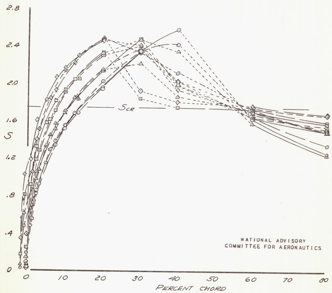
FIGURE 53.- EFFECT OF LEADING-EDGE MODIFICATIONS ON PRESSURE DISTRIBUTION ON UPPER SURFACE. WING STATION 35.638, M=0.75 .
