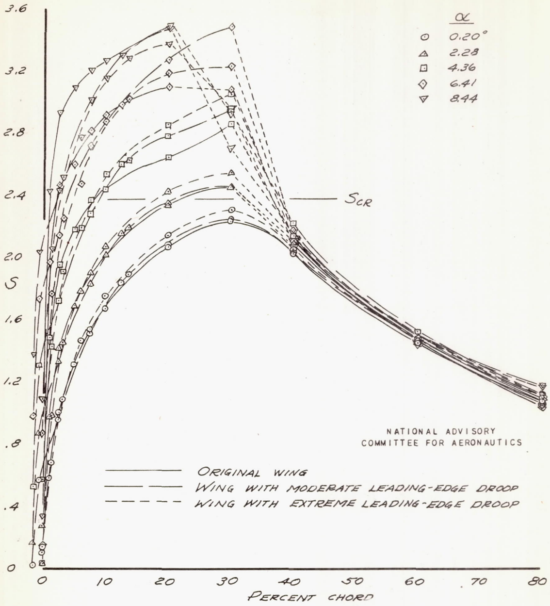
FIGURE 51.- EFFECT OF LEADING-EDGE MODIFICATIONS ON PRESSURE DISTRIBUTION ON UPPER SURFACE. WING STATION 35.638, M=0.60 .
