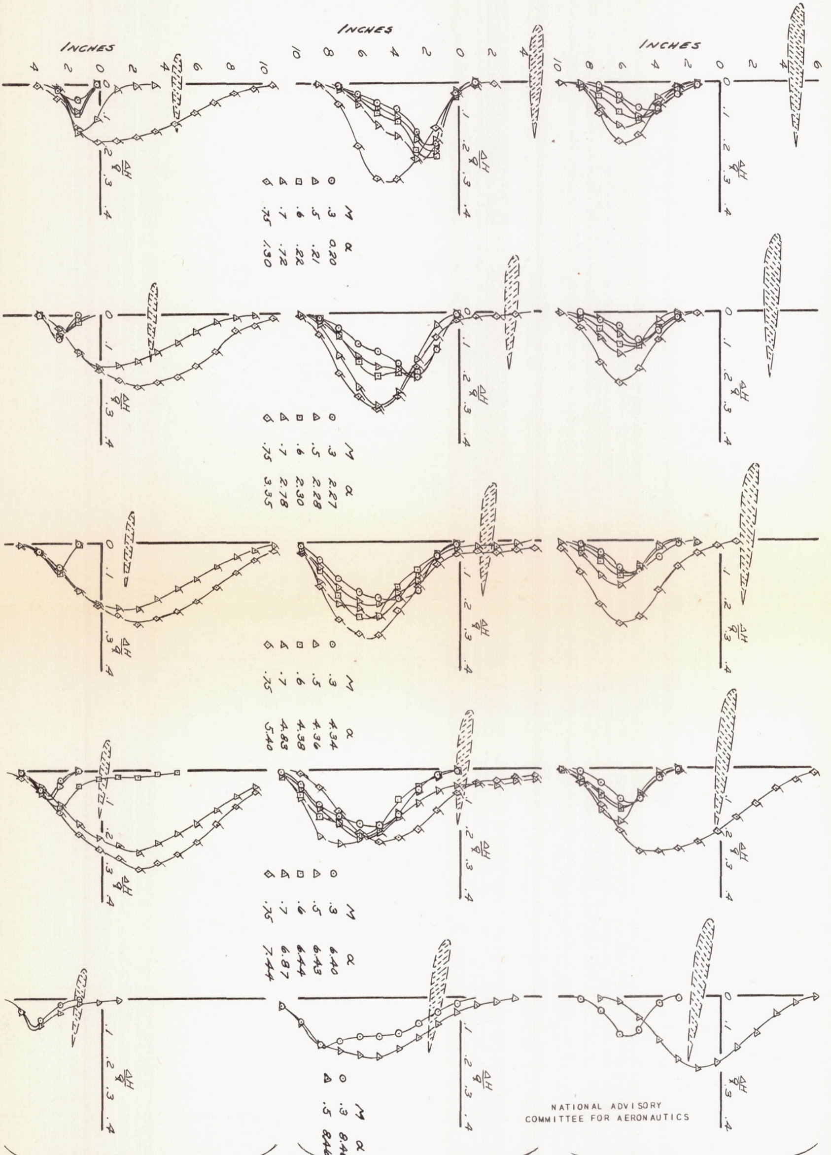
TAIL STATION 16.6 TAIL STATION 9.825 TAIL STATION 4.575 FIGURE 35. - POSITION OF WING WAKE RELATIVE TO THE TAIL AT VARIOUS MACH NUMBERS AND ANGLES OF ATTACK. WING, NACELLES, FUSELAGE, TURRETS AND SIGHTING DOMES, AND SMALL 45° TAPERED FLAPS ALONG REAR SPAR BETWEEN FUSELAGE AND INBOARD NACELLES.
