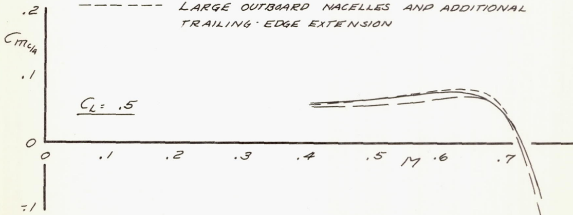
FIGURE 44. - PITCHING-MOMENT COEFFICIENTS WITH SMALL OUTBOARD NACELLES, LARGE OUTBOARD NACELLES, AND LARGE OUTBOARD NACELLES WITH ADDITIONAL TRAILING-EDGE EXTENSIONS.
