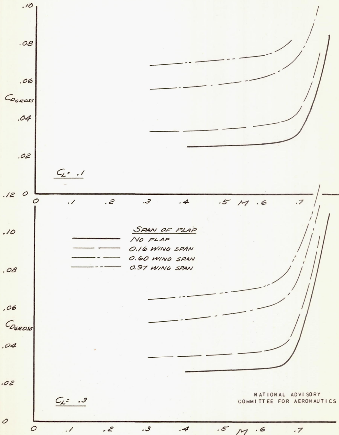
FIGURE 30(a). - EFFECT OF AUXILIARY FLAP SPAN ON DRAG COEFFICIENT. SMALL TAPERED FLAPS, 45°, INTERMEDIATE POSITION. LIFT COEFFICIENT = 0.1 AND 0.3.
