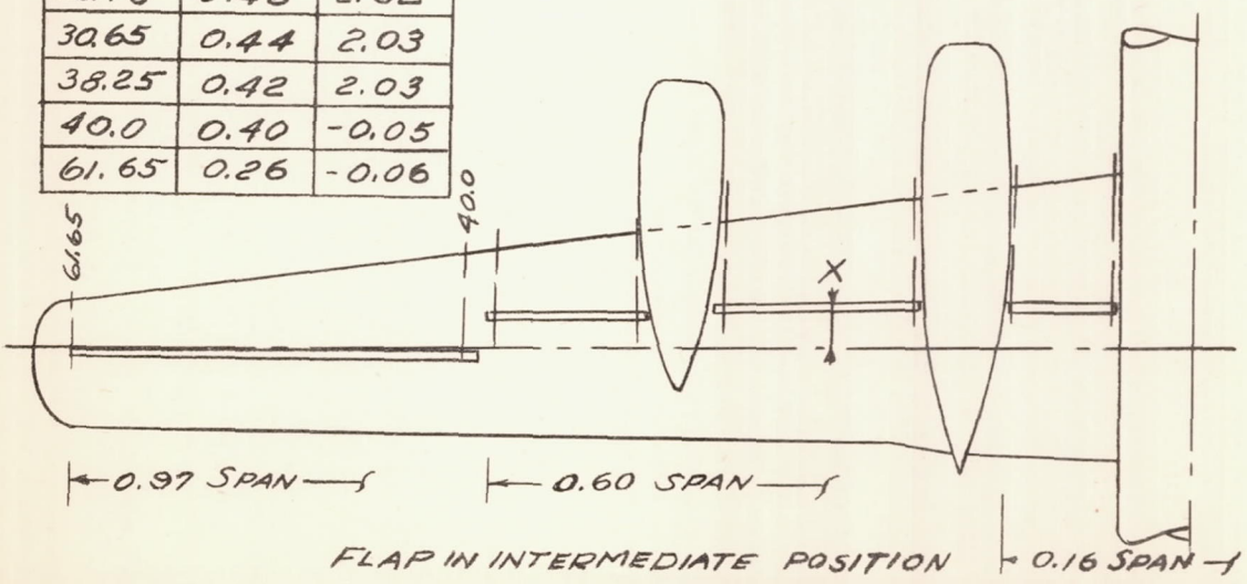
FIGURE 4. - LOCATION AND DIMENSIONS OF 45° SMALL TAPERED FLAP ALONG FORWARD SPAR AND IN INTERMEDIATE POSITION.
