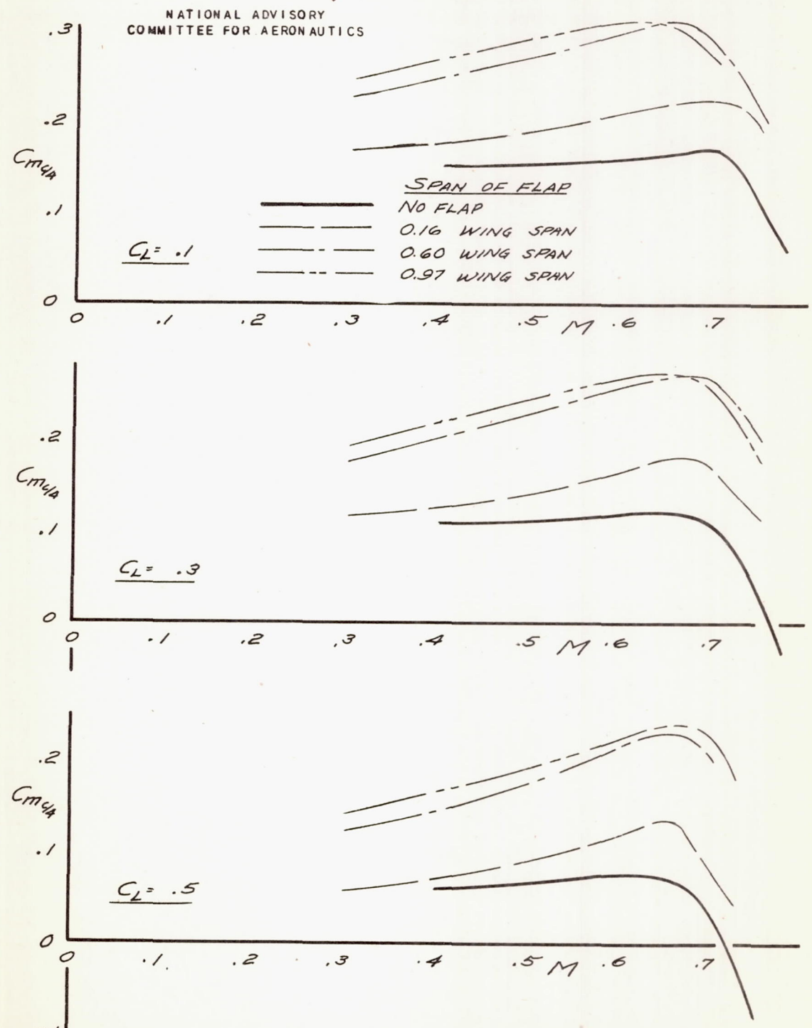
FIGURE 28.- EFFECT OF AUXILIARY FLAP SPAN ON PITCHING-MOMENT COEFFICIENT. SMALL TAPERED FLAPS, 45°, INTERMEDIATE POSITION.
