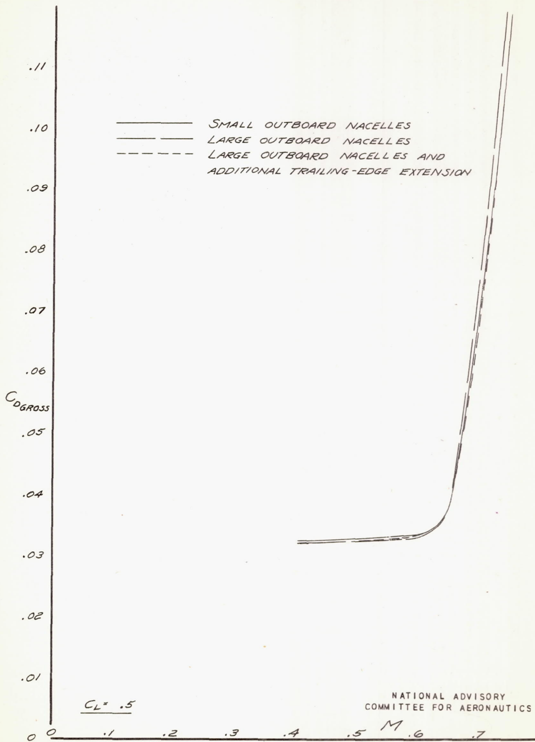
FIGURE 46 (c). - DRAG COEFFICIENTS WITH SMALL OUTBOARD NACELLES, LARGE OUTBOARD NACELLES, AND LARGE OUTBOARD NACELLES WITH ADDITIONAL TRAILING-EDGE EXTENSIONS. LIFT COEFFICIENT = 0.5.
