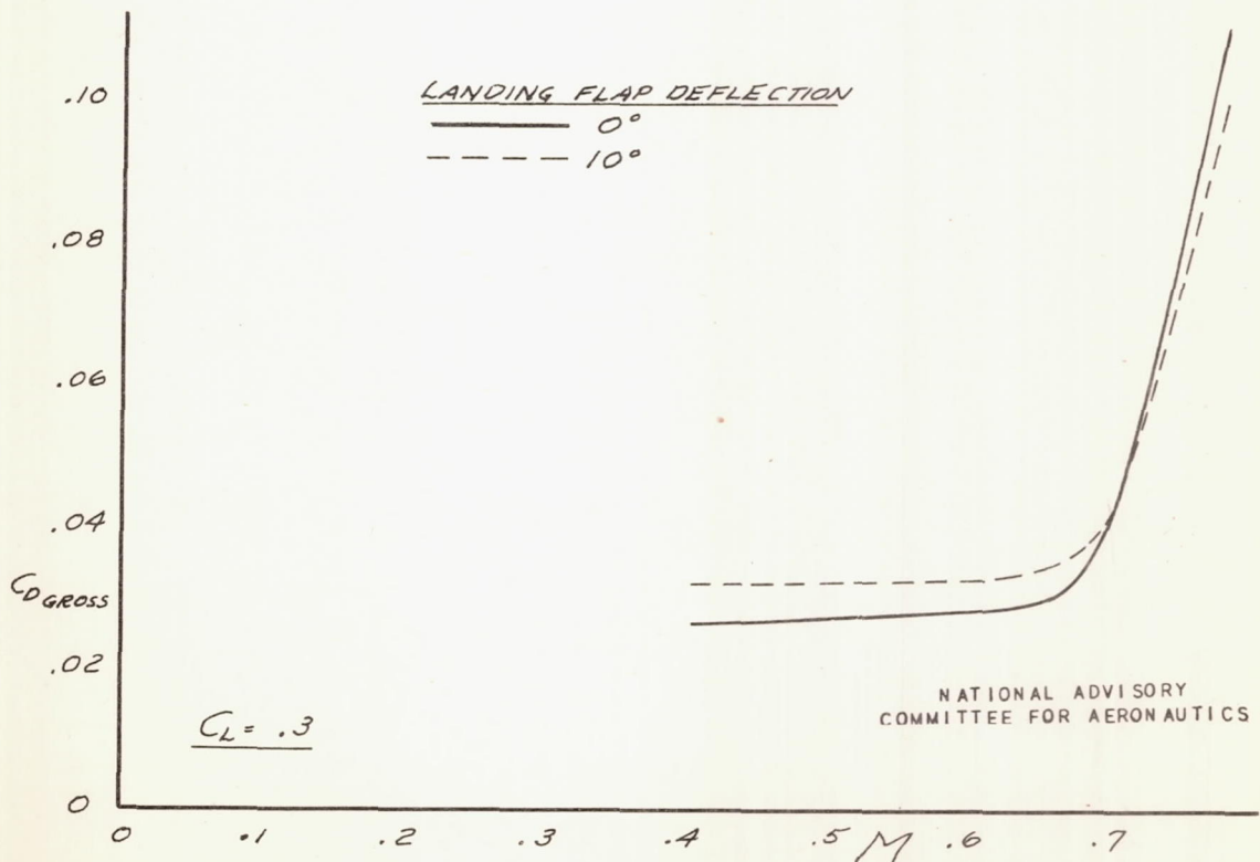
FIGURE 18 (a). - EFFECT OF 10° LANDING FLAP DEFLECTION ON DRAG COEFFICIENT FOR CONSTANT LIFT COEFFICIENT. LIFT COEFFICIENT = 0.1 AND 0.3
