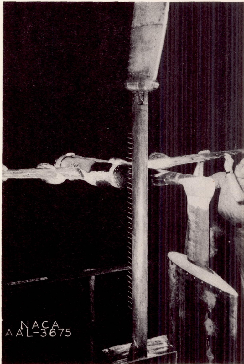
Figure 12.- Wake-survey rake.
