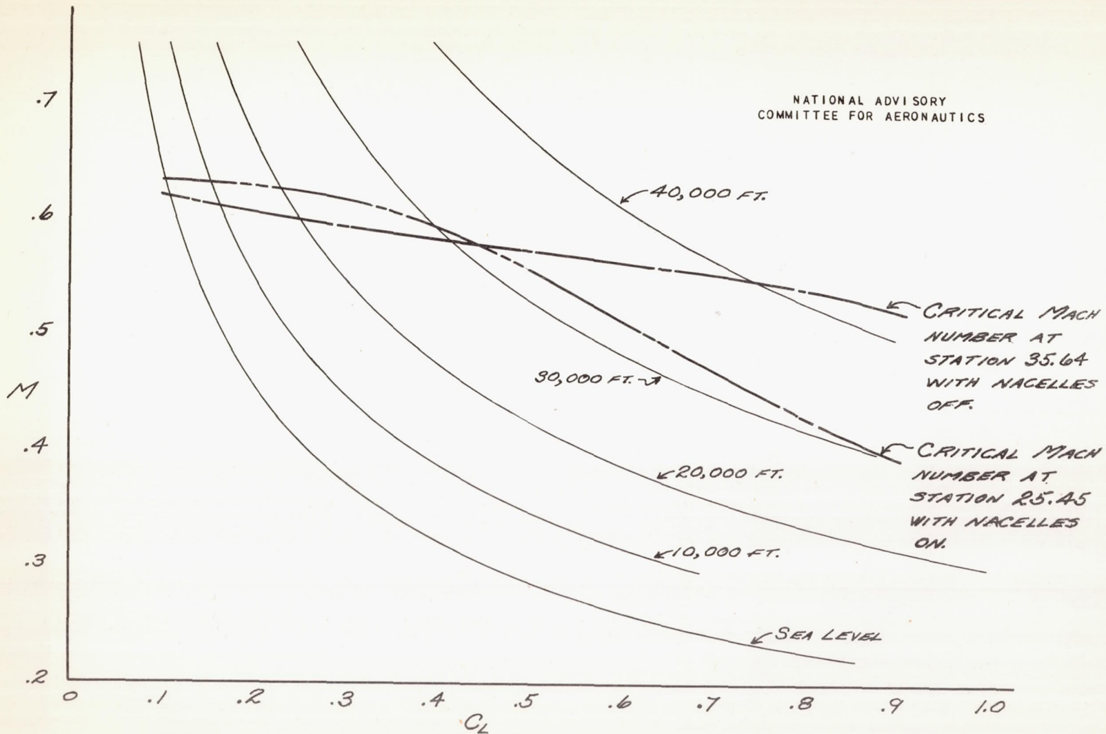
FIGURE 40. - CRITICAL MACH NUMBER OF WING ALONE AND WITH NACELLES. LEVEL FLIGHT CONDITIONS AT A WING LOADING OF 61.25 POUNDS PER SQUARE FOOT.
