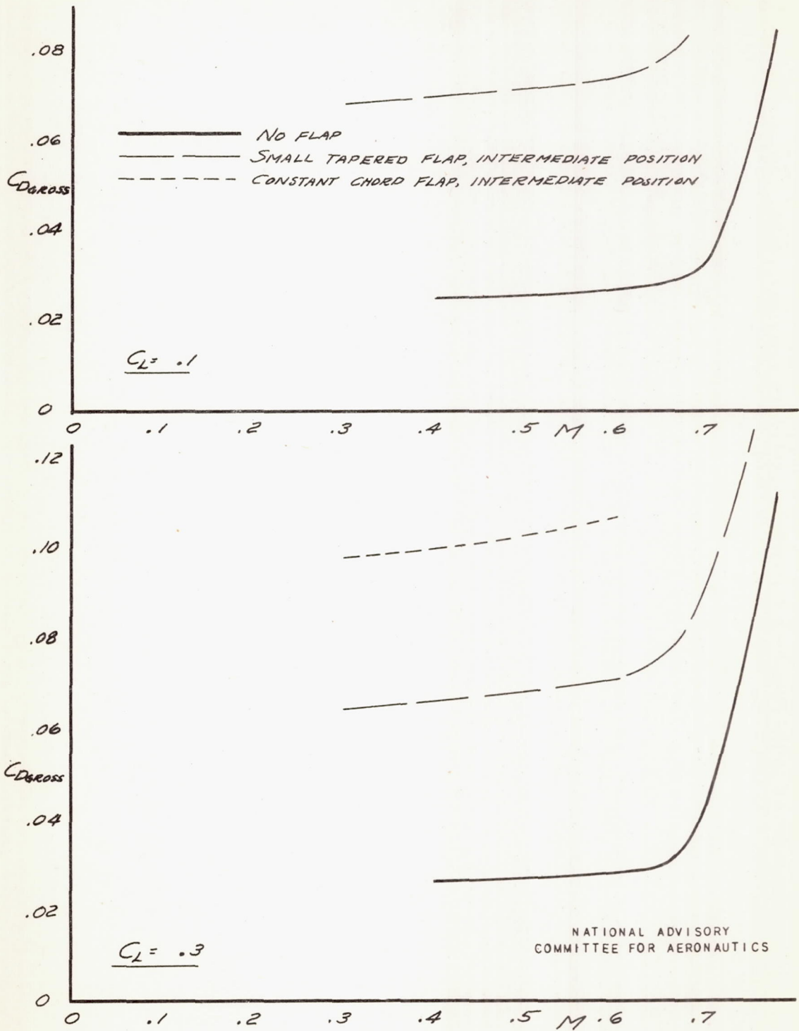
FIGURE 27(a). - EFFECT OF 0.97 SPAN 45^\circ AUXILIARY FLAPS ON DRAG COEFFICIENT. LIFT COEFFICIENT = 0.1 AND 0.3.
