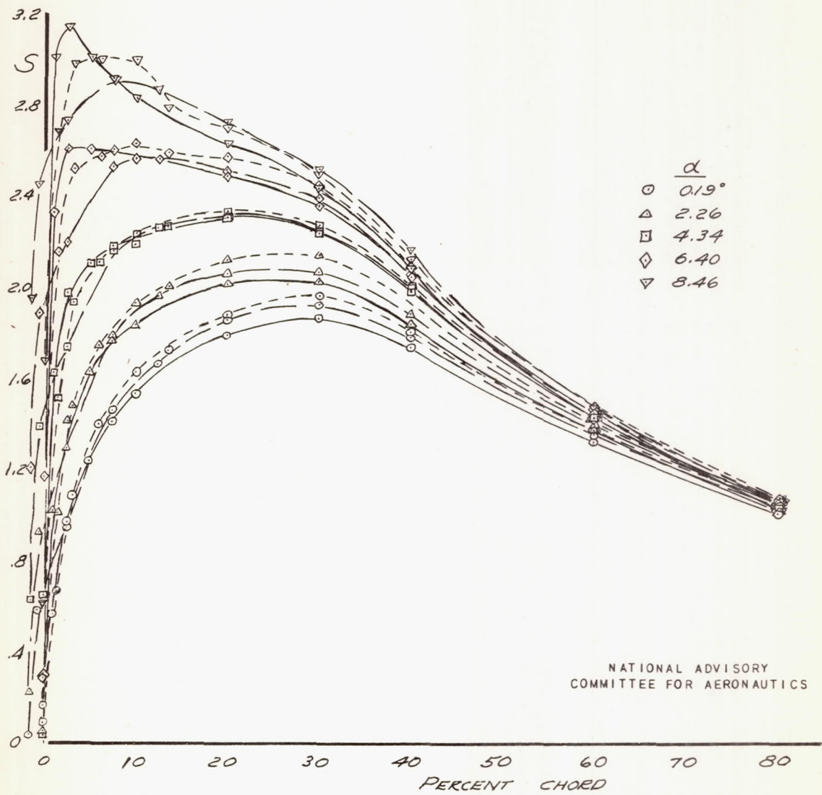
FIGURE 49. - EFFECT OF LEADING-EDGE MODIFICATIONS ON PRESSURE DISTRIBUTION ON UPPER SURFACE. WING STATION 35.638, M = 0.40 .
