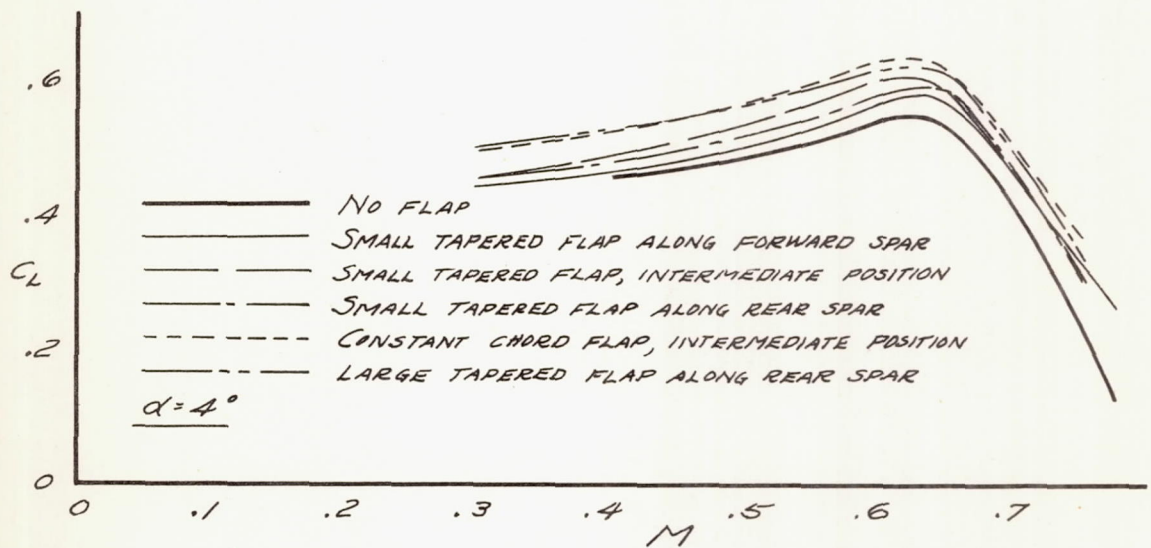
FIGURE 20. - EFFECT OF 0.16 SPAN 45^\circ AUXILIARY FLAPS ON LIFT COEFFICIENT.
