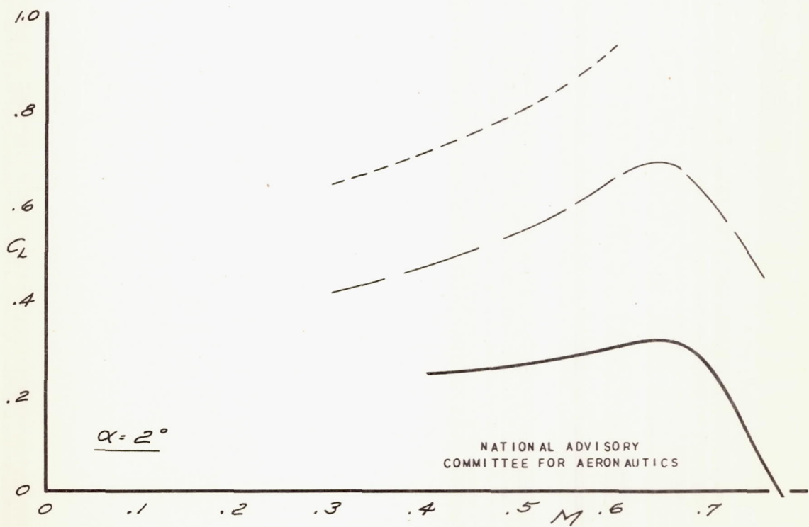
FIGURE 26 (a). - EFFECT OF 0.97 SPAN 45^\circ AUXILIARY FLAPS ON LIFT COEFFICIENT. ANGLE OF ATTACK = 0^\circ AND 2^\circ .
