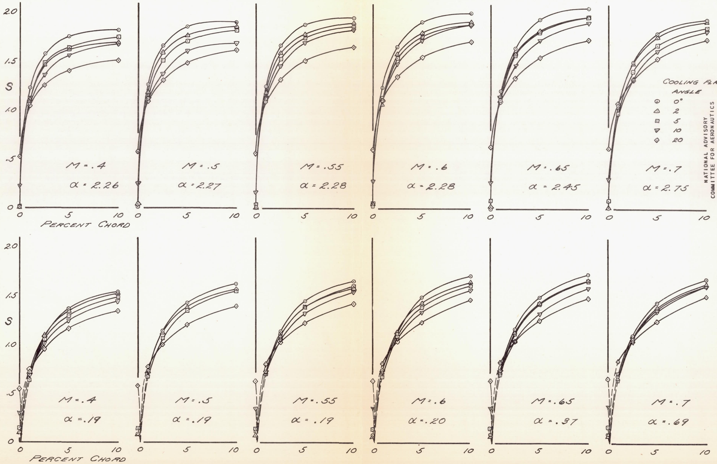
FIGURE 41 (a). - PRESSURE DISTRIBUTION ON UPPER SURFACE OF WING AT DIFFERENT COOLING FLAP DEFLECTIONS. WING STATION 15.476; UNCORRECTED ANGLE OF ATTACK 0° AND 2°.
