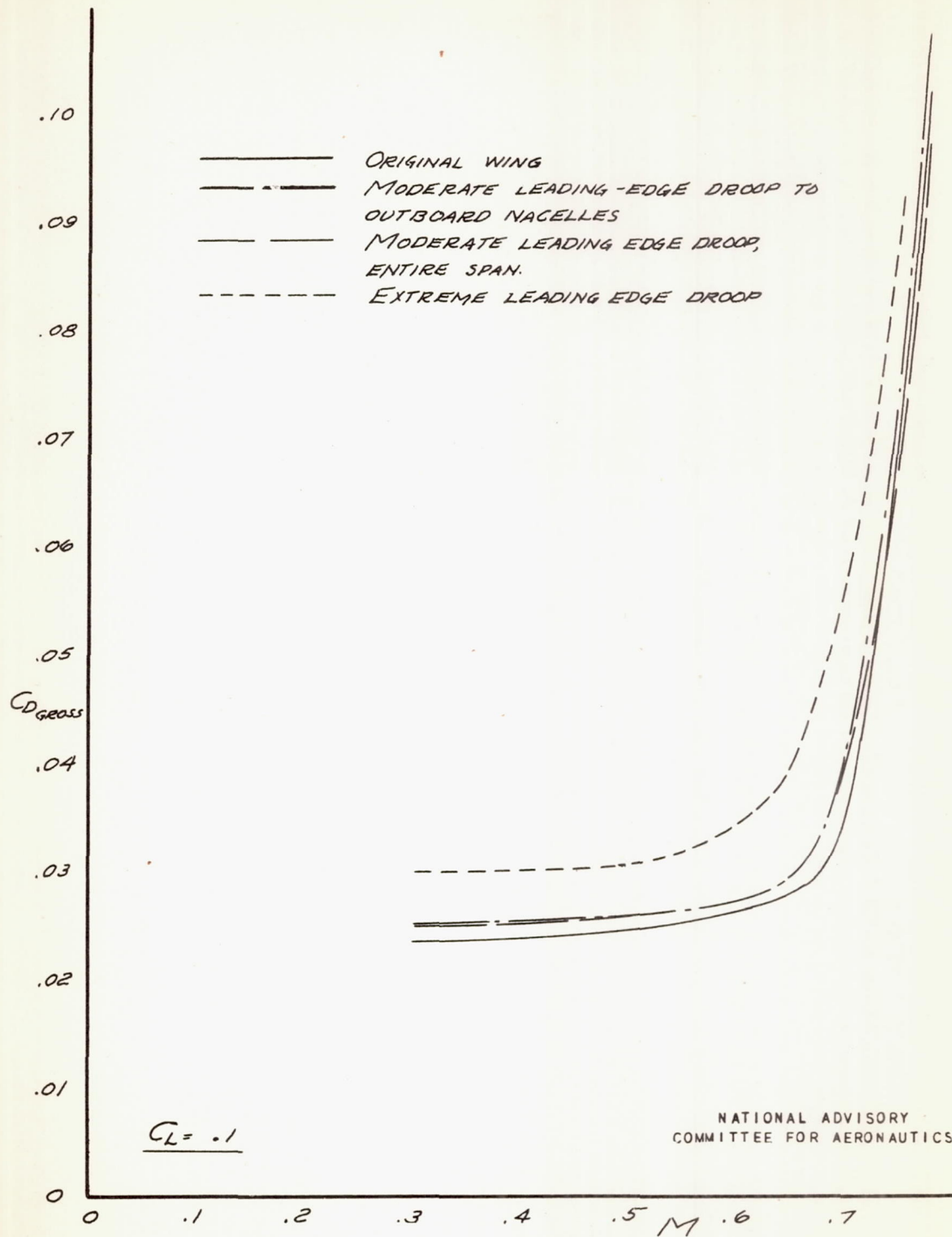
FIGURE 48 (Q). - EFFECT OF LEADING-EDGE MODIFICATIONS ON DRAG COEFFICIENTS. LIFT COEFFICIENT = 0.1.
