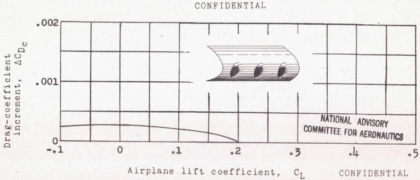
Figure 9.- Drag increments of gun ports on wing of F4U-1 airplane in Langley full-scale tunnel. R = 7.6 \times 10^6 .
