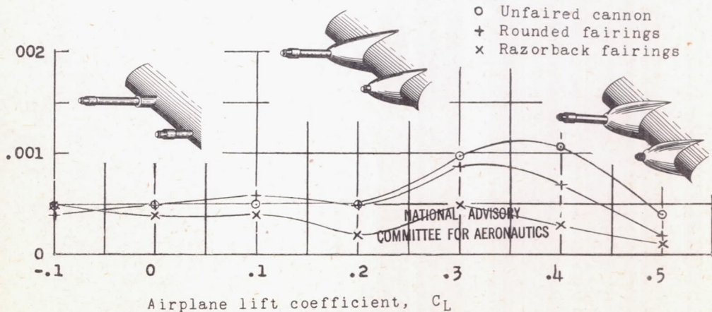
(c) Cannon installations on model of XF6F airplane in Langley 19-foot pressure tunnel. R = 6.15 \times 10^6 .
