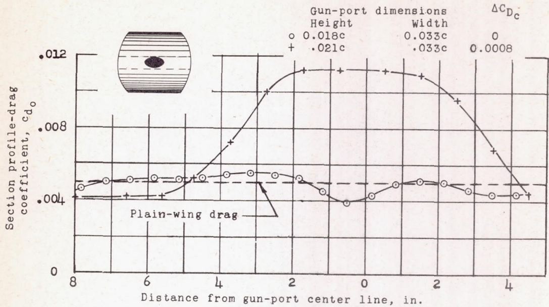
(a) Gun ports on chord line.
