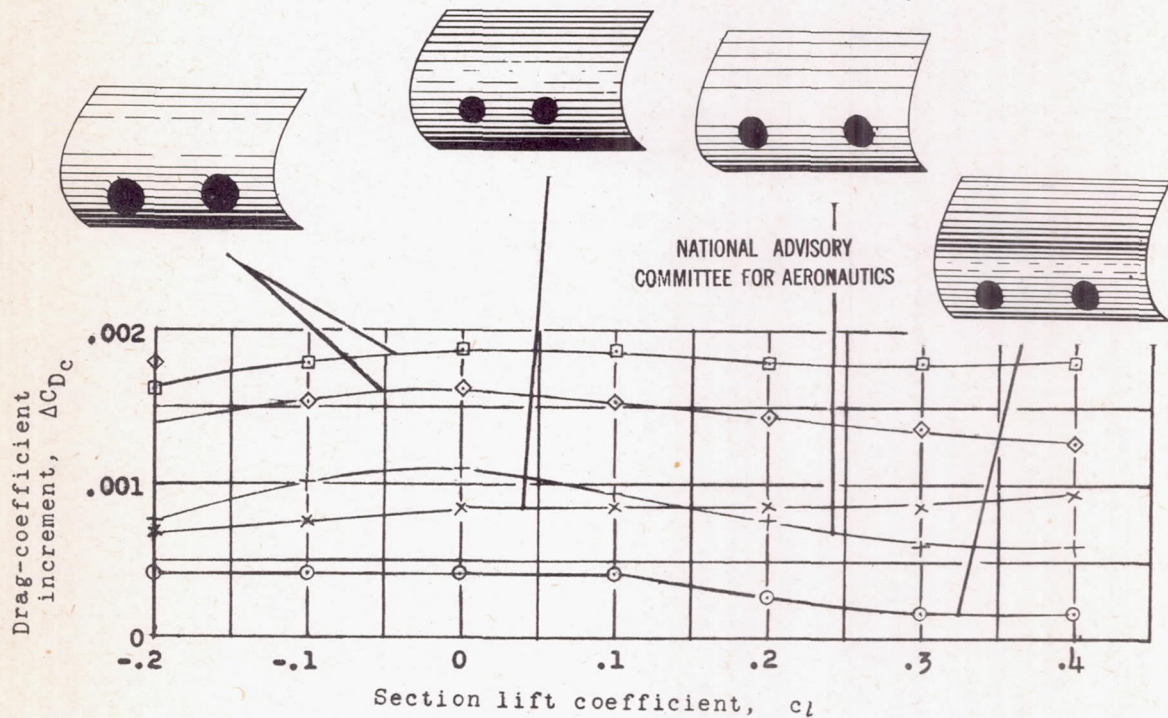
Figure 16.- Drag increments of gun ports on model of wing of XA-41 airplane in Ames 7- by 10-foot tunnel. No flow through ports. R = 6.35 \times 10^6 .
