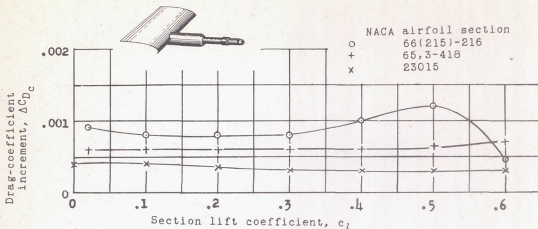
(a) Drag increments of cannon on three NACA airfoil sections.
