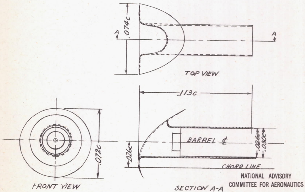
(c) Typical gun sleeve.
