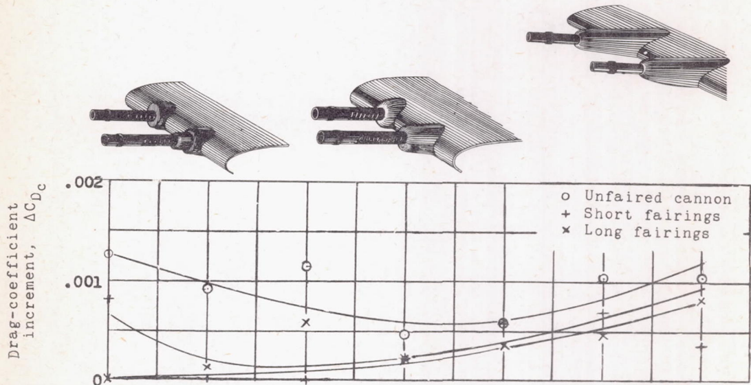
(b) Cannon on model of XF4U-1 airplane in Langley 19-foot pressure tunnel. R = 2.75 \times 10^6 .
