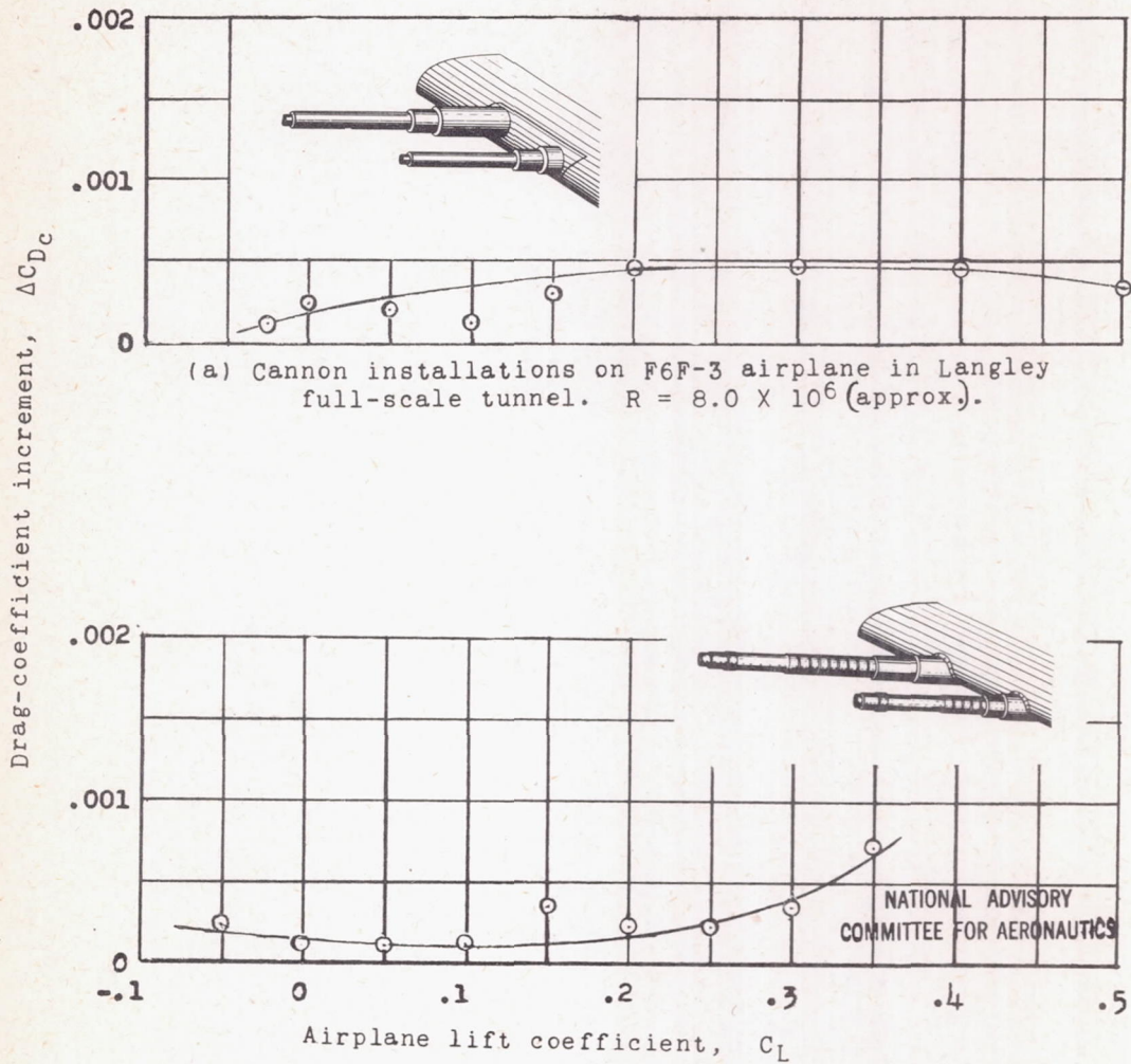
(b) Cannon on F4U-1 airplane in Langley full-scale tunnel. R = 7.6 \times 10^6 .
