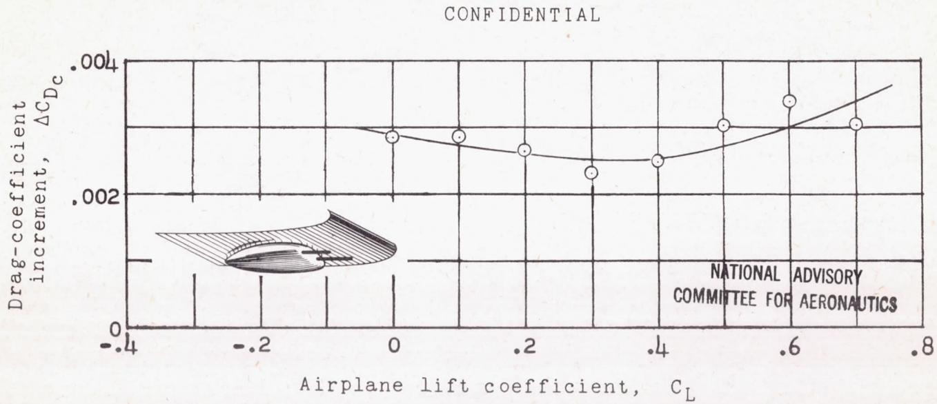
Figure 27.- Drag increments of gun installation on model of XA-26 airplane in Langley 19-foot pressure tunnel. R = 3.6 \times 10^6 .
