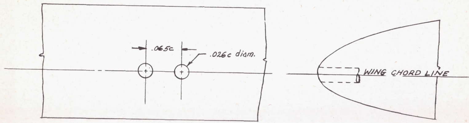
Figure 15.- Machine-gun ports on model of wing of XA-41 airplane. (These holes also tested centered 0.0082c and 0.0165c below chord.)
