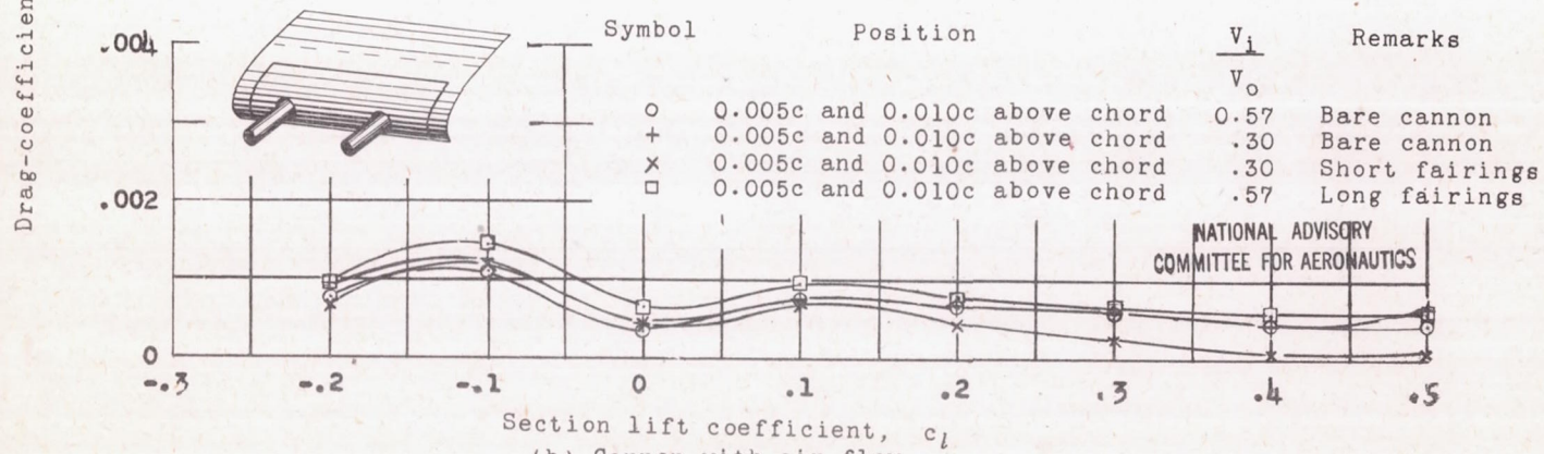
(b) Cannon with air flow.
