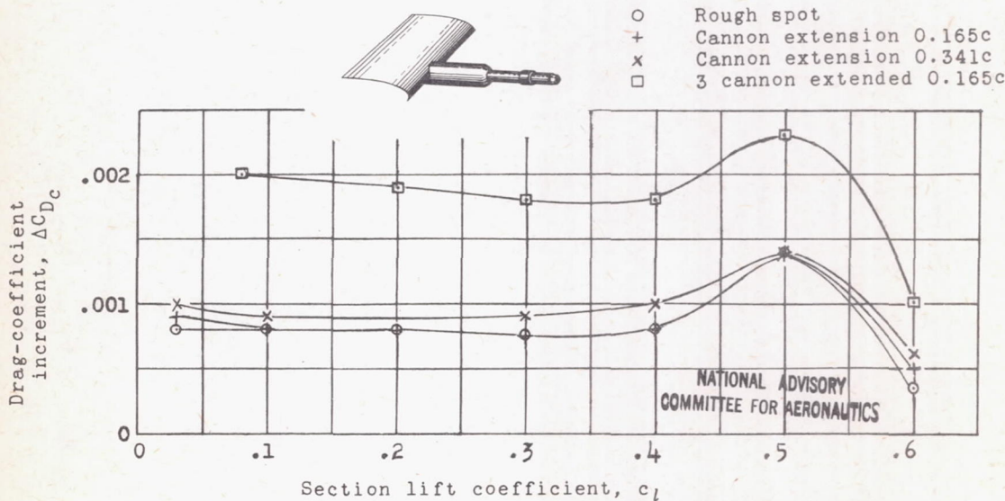
(b) Drag increment of two cannon extensions compared with drag increment of rough spot on NACA 66(215)-216 airfoil section.
