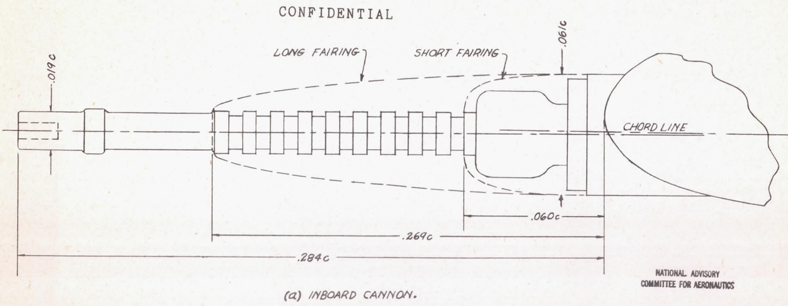
Figure 35.- Cannon installations on model of XF4U-1 airplane.
