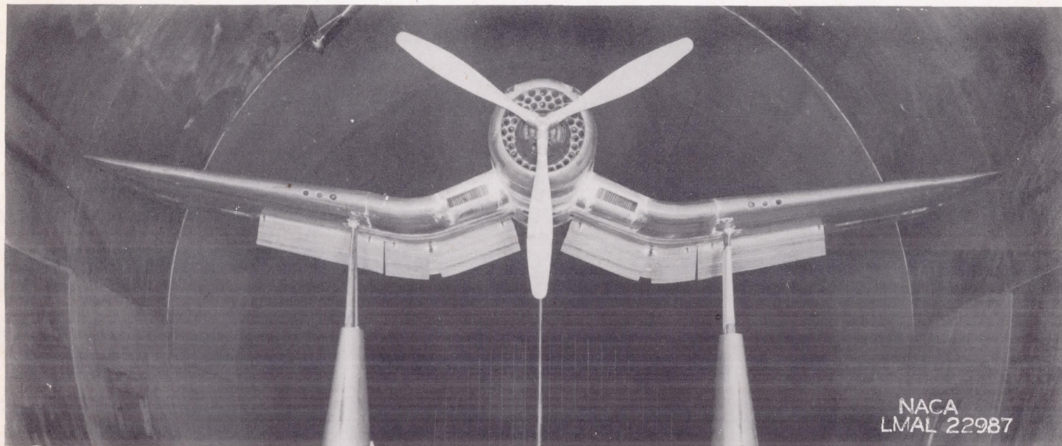
Figure 6.- Gun ports on \frac{1}{2.75} -scale model of XF4U-1 airplane. Gun ports are of 1-inch diameter with exits ahead of flap.
