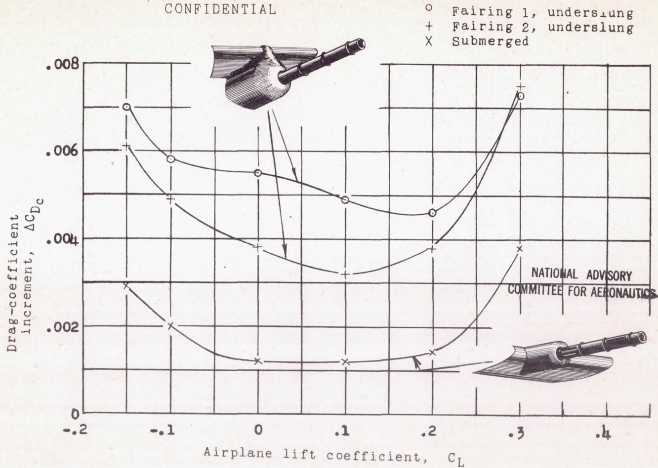
Figure 30.- Cannon drag increments on XF2A-2 airplane in Langley full-scale tunnel. R = 5.5 \times 10^6 .
