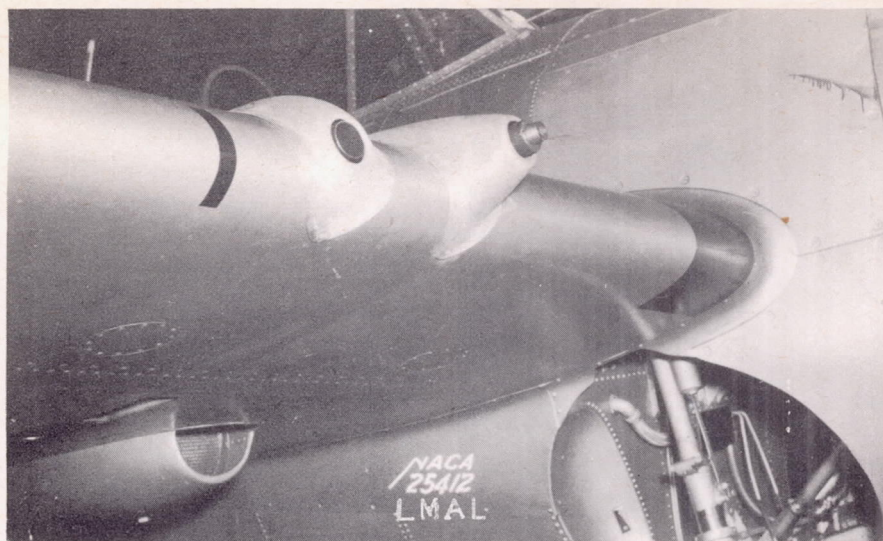
(c) View of fairing 2 (wide) on submerged gun and Grumman fairing on projecting gun. Both fairings provide space around gun barrel for cooling air.
