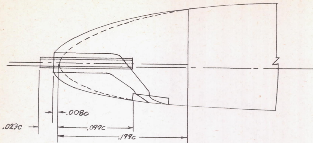
(a) Short fairings and cannon.
