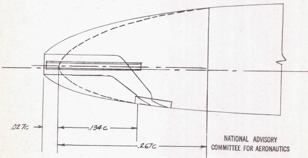
(b) Long fairings and cannon.
