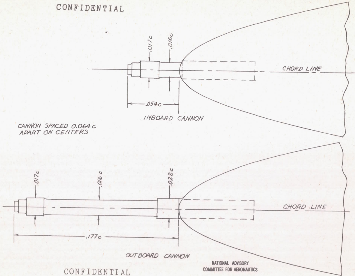
Figure 34.- Cannon installations on model of XF6F airplane.
