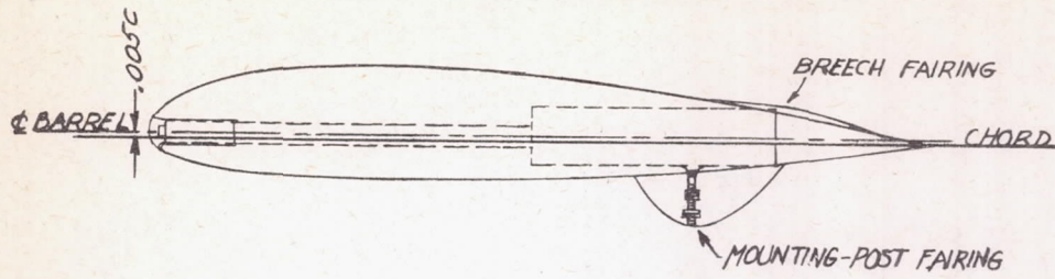
(a) Low flush gun position.
