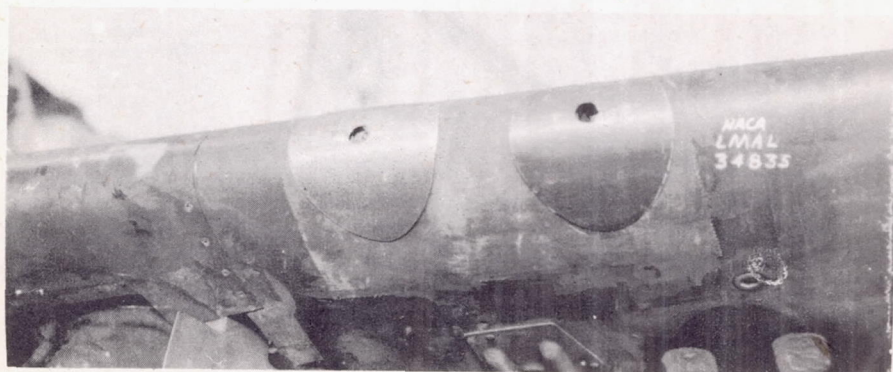
(c) Gun ports covered with metal plates having holes of 5.3-percent thickness to allow passage of bullet.
