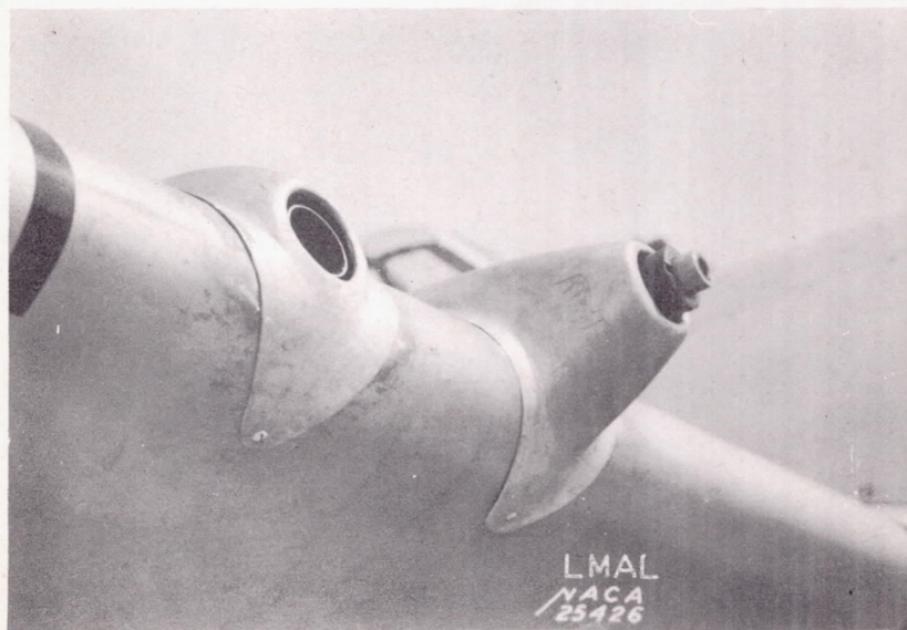
(d) View of fairing 3 (narrow) on submerged gun and Grumman fairing on projecting gun. Both fairings provide space around gun barrel for cooling air.
