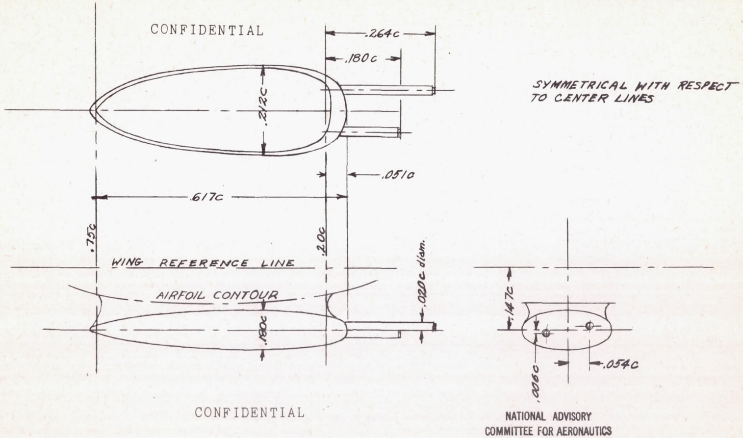
Figure 26.- Machine-gun mount on model of XA-26 airplane.
