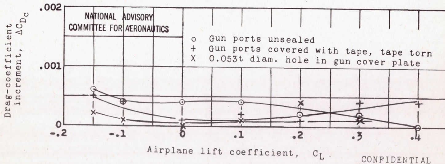
Figure 18.- Drag increments of several gun-port installations on P-51B airplane in Langley full-scale tunnel. R = 6.5 \times 10^6 .
