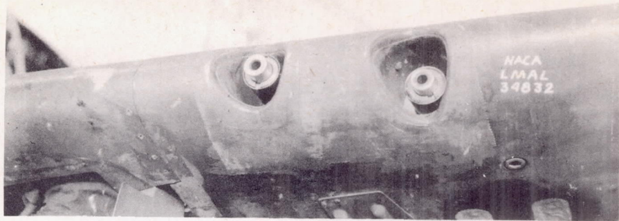
(a) Gun ports open.
