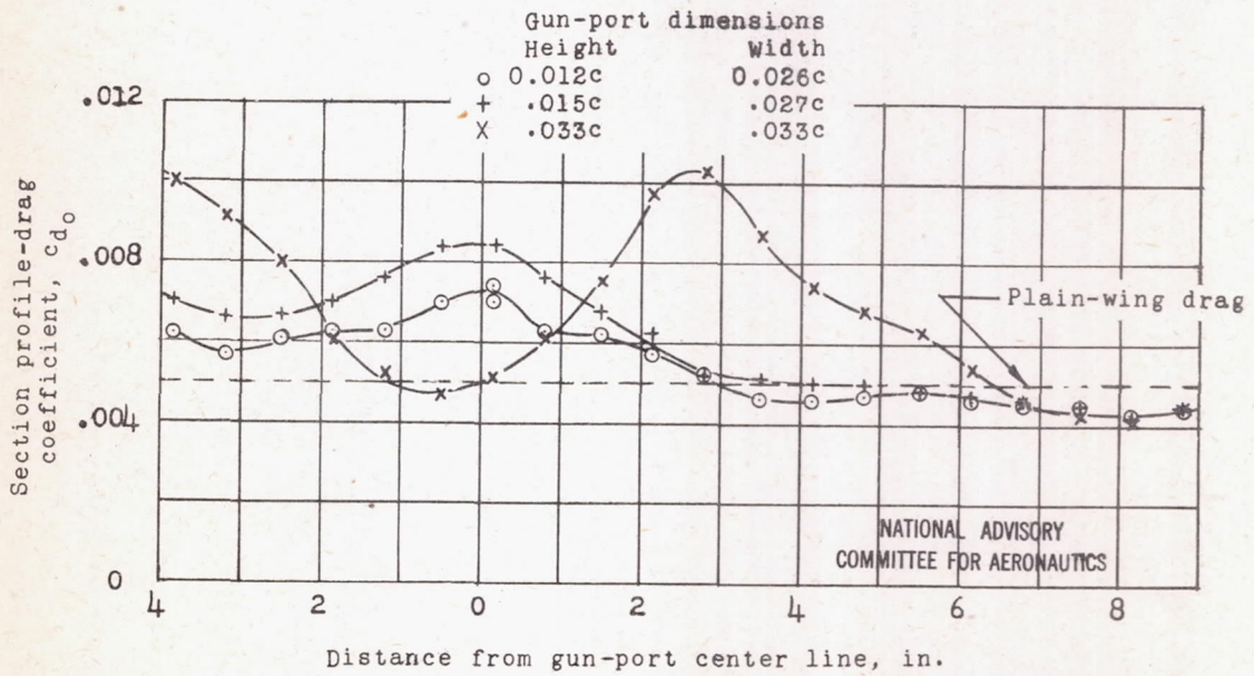
(b) Gun ports 0.014c below chord line.
