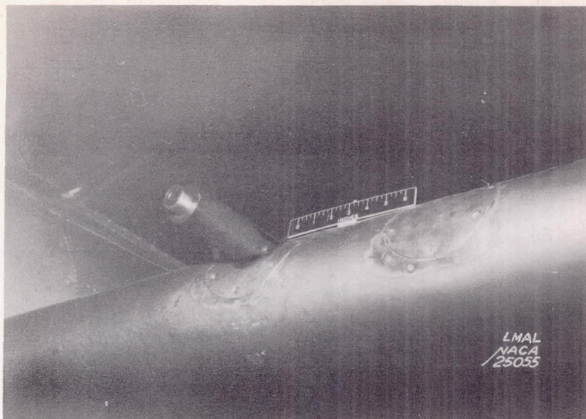
(a) View of projecting gun in unfaired condition with submerged gun removed.
