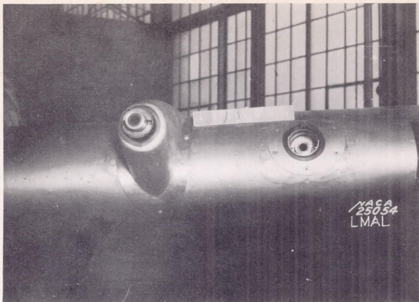
(e) View of submerged gun in unfaired condition and projecting gun with Grumman fairing. Rubber grommets installed around edges of fairing and wing opening.
