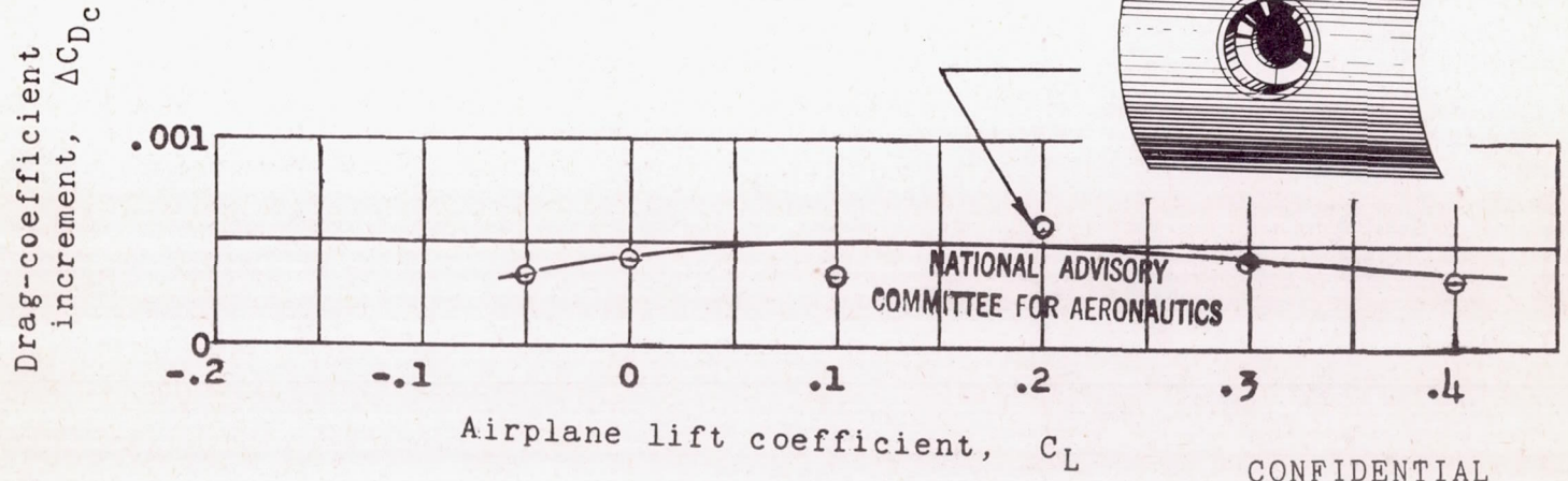
Figure 5.- Drag increments of gun ports on wing of model of modified XP-41 airplane in Langley 19-foot pressure tunnel. R = 6.15 \times 10^6 .
