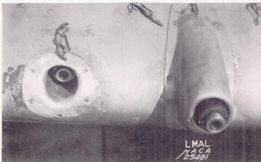
(f) View of faired wing opening for submerged gun and Grumman fairing on projecting gun. Both fairings provide space around gun barrels for cooling air.
