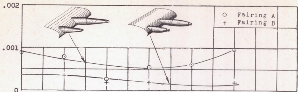
(a) Cannon installations on model of XF14C-2 airplane in Langley 19-foot pressure tunnel. R = 5.5 \times 10^6 .
