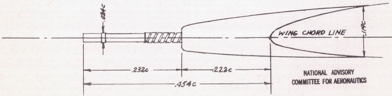
Figure 39.- Cannon installation on P-51B airplane.
