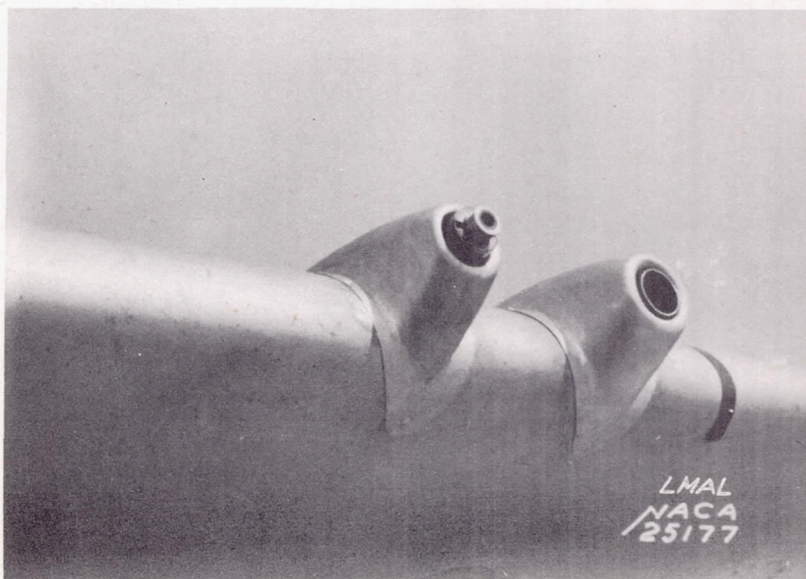
(b) View of fairing 1 on submerged gun and Grumman fairing on projecting gun. Both fairings provide space around gun barrel for cooling air.
