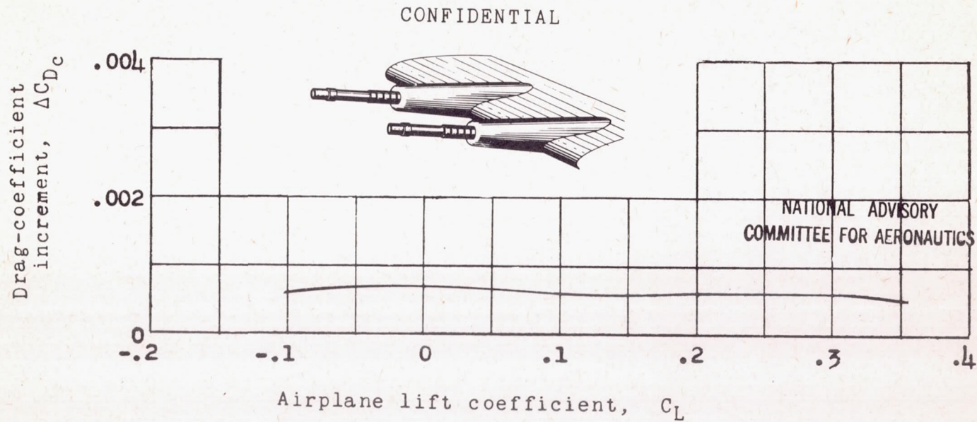
Figure 40.- Drag increments of cannon on P-51B airplane in Langley full-scale tunnel. R = 6.0 \times 10^6 .
