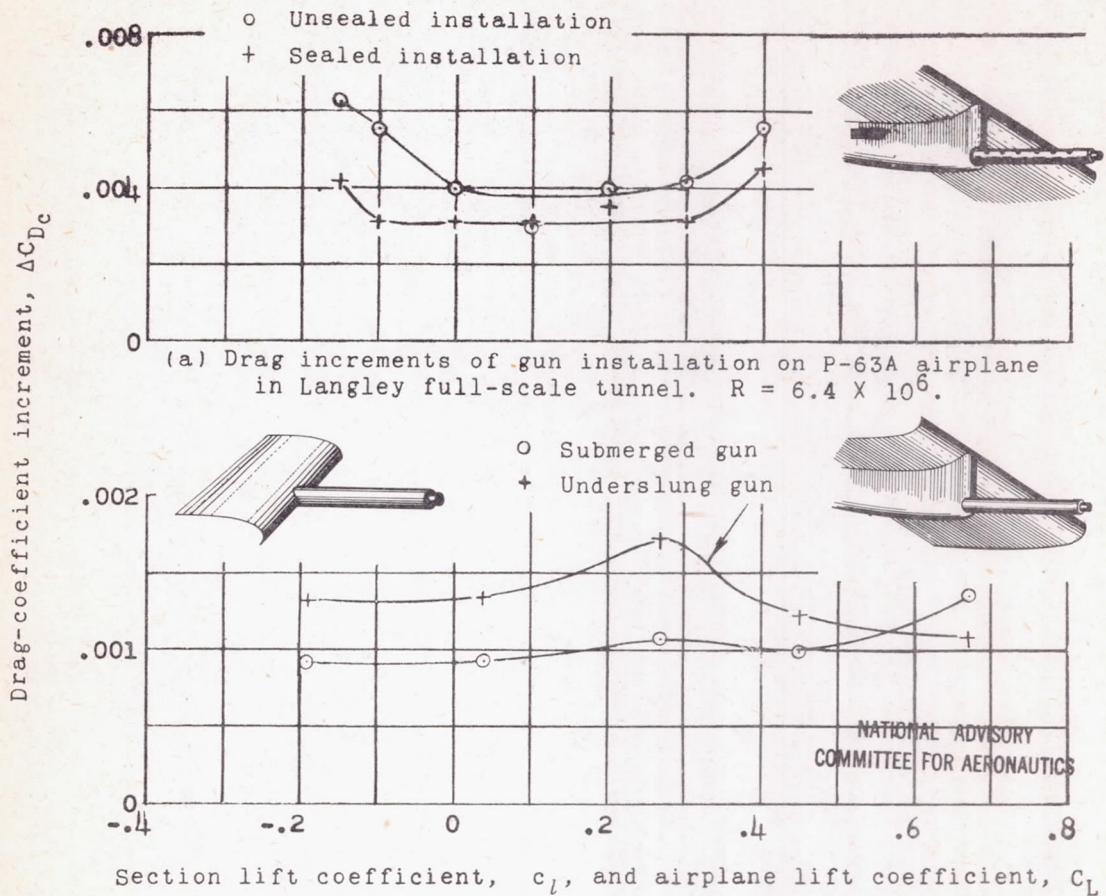
(a) Drag increments of gun installation on P-63A airplane in Langley full-scale tunnel. R = 6.4 \times 10^6 . (b) Drag increments of two gun installations on model of wing of XP-63 airplane in Langley two-dimensional low-turbulence pressure tunnel. R = 6.0 \times 10^6 .
